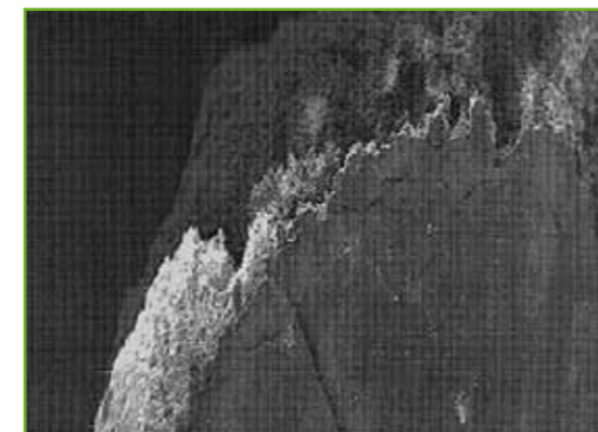
Electron microscope scan: White areas: latent hydraulic compounds which penetrated into the pore structure of the substrate – and reacted to form a pore sealing solid body.
